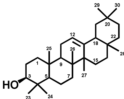
Fig. 1. Purified compound 1 was characterized as \beta -amyrin.
