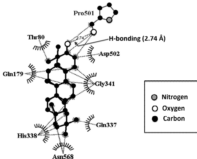
Fig. 3. Ligplot 2D map of interaction between mice COX-2- and β-amyrin. Hydrophobic contacts are represented by arcs with radiating spokes. Atom with dots is the corresponding atom involves in hydrophobic interaction.
